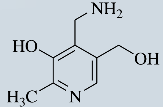
pyridoxamine
