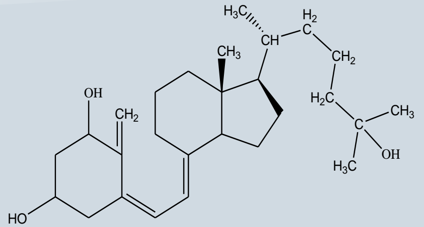
1,25-dihydroxyvitamin D 3
