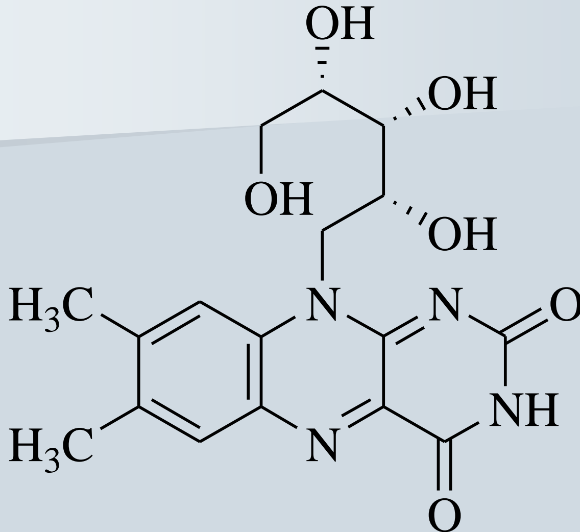
Riboflavin
