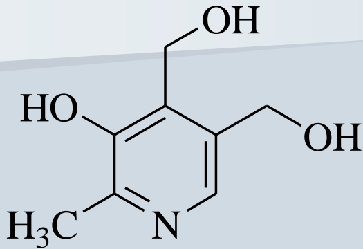
pyridoxol
