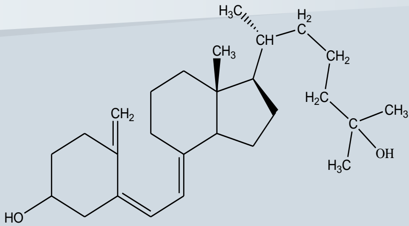
25-hydroxyvitamin D 3
