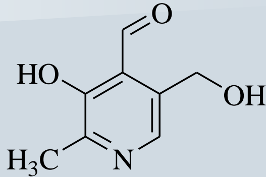
pyridoxal
